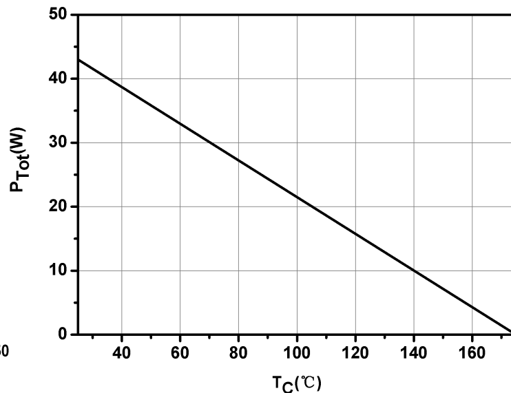
Fig.6-Power Derating
