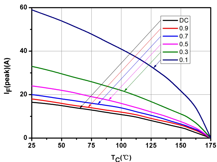
Fig.7-Current Derating
